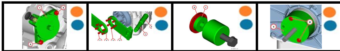
2992380 2992475 2992452 2992214 Turning Gear Locking Device Counter Holder Crank Seal Ring Ass (Opposite Flywheel) Assembly Tool (Flywheel Side)
