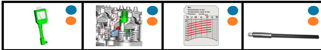
1899034 Compression Gauge (With Adapter) 2992018 Connection Piece (Comp. Gauge) 1899193 Compression Chart Sheets 1899185 Torque Handle Insert
