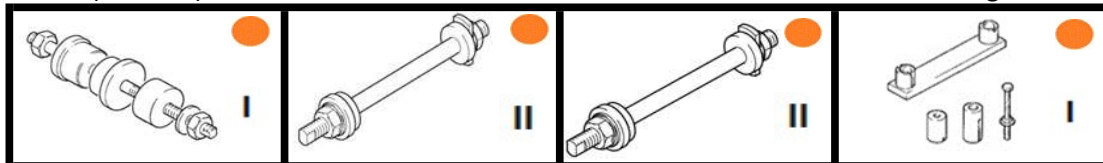
2992241 2992245 2992249 2992296 Camshaft Bearing Installer Camshaft Bearing Remover Camshaft Bearing Remover Piston Cooling Nozzel Alignment Tool
