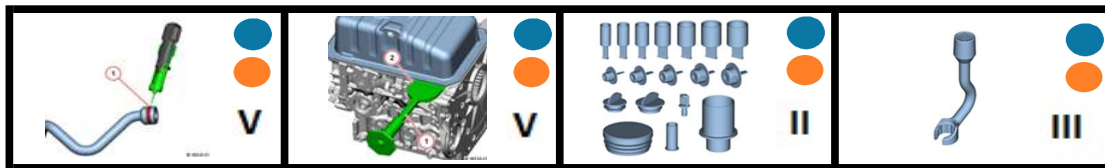
2992127 2992301 1899368 2992477 Disassembly Tool Separating Tool Locking Plugs / Caps Special Wrench (Fuel Line)
